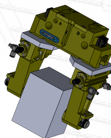
Gripper Solutions
